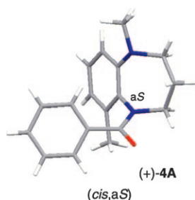
Figure 2: X-ray crystal structure of (+)- 4A (= cis,aS ) generated from the CIF file.
